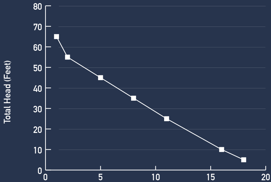
Flow Rate (GPM - Gallons Per Minute) Performance based on using 1/3 hp, 1725 rpm motor
