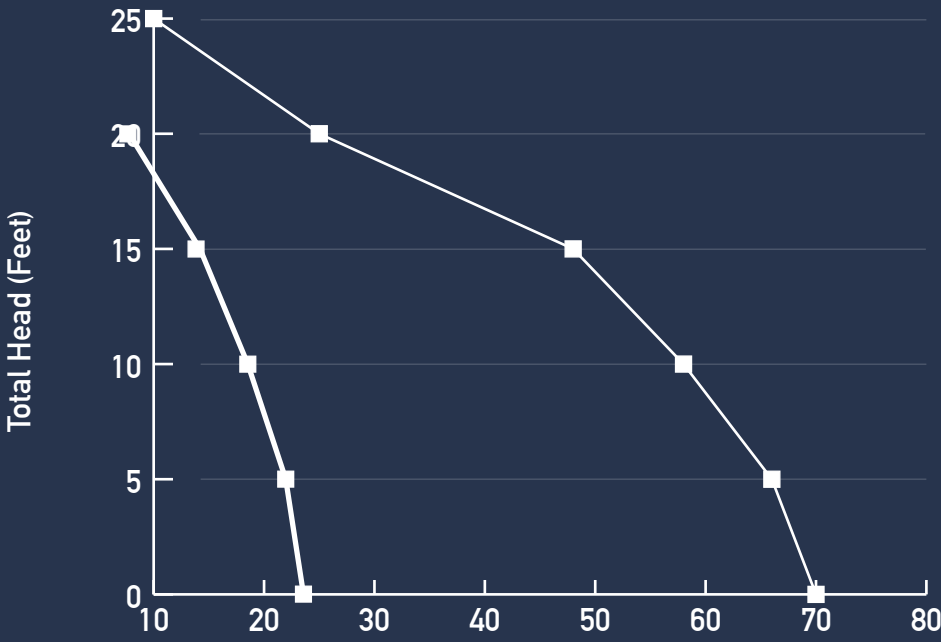
BACKUP - 92910 | PRIMARY - 92511 low Rate (GPM - Gallons Per Minute)
