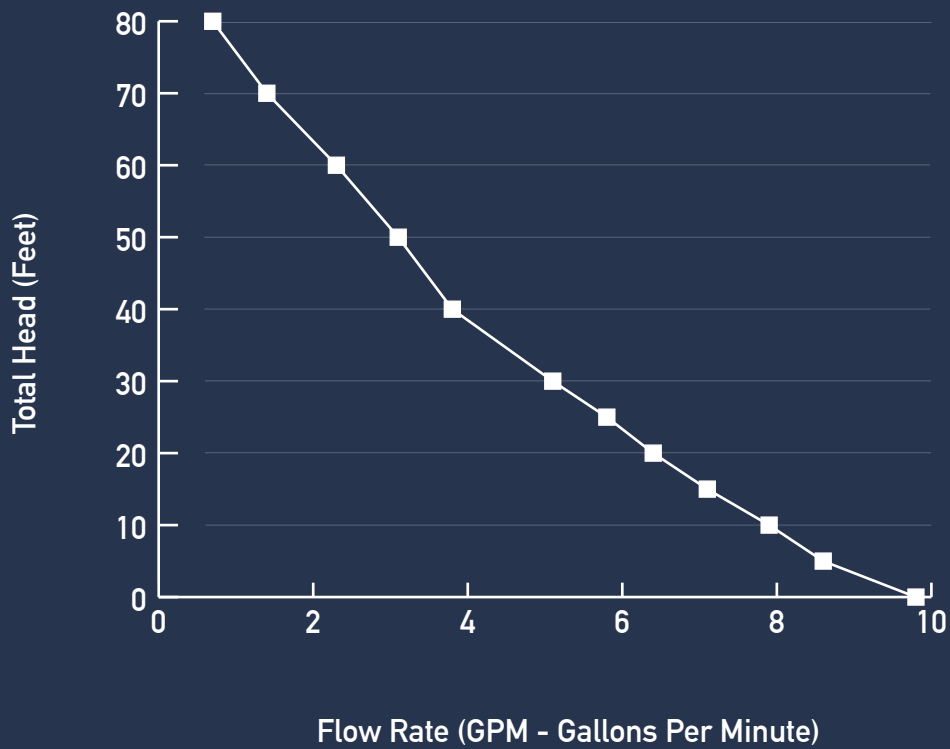
Approximate gallons per minute output at 40 psi (Maximum pressure 61 psi)
