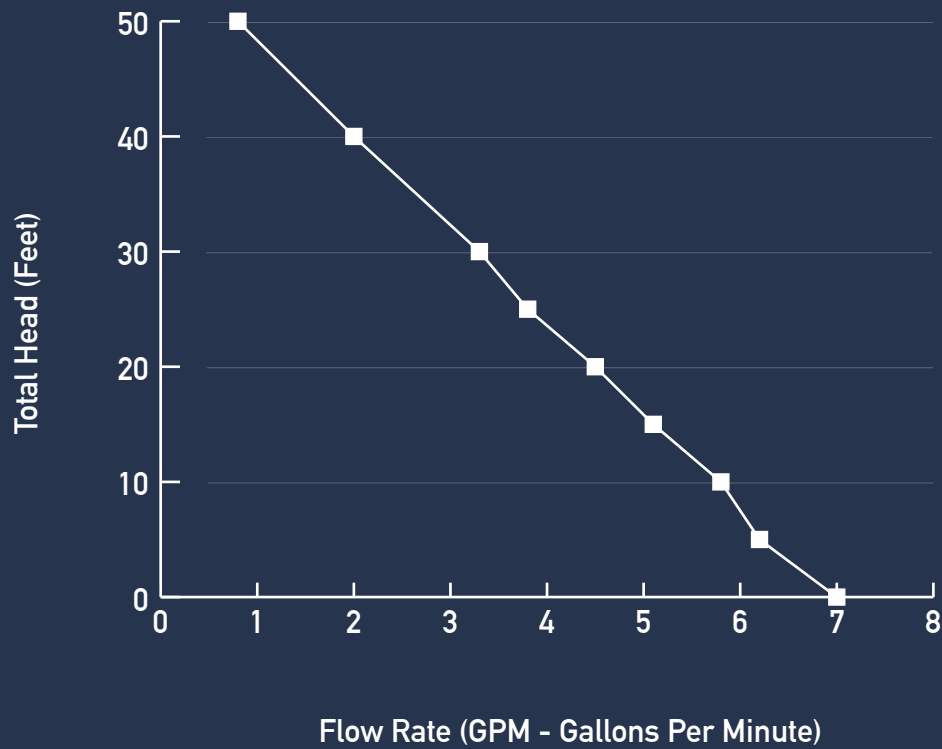
Approximate gallons per minute output at 40 psi (Maximum pressure 58 psi)
