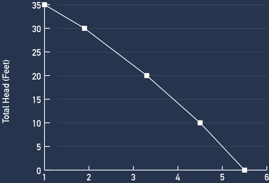
Flow Rate (GPM - Gallons Per Minute) (Performance based on fully charged 12 volt battery, sold separately)
